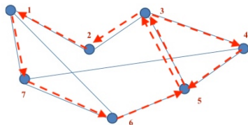
Circuito: 1, 7, 6, 5, 3, 4, 5, 3, 2, 1
